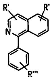
arylquinolines
