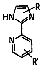
pyridylimidazoles
