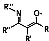
iminoacetates
