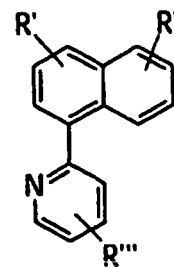
pyridynaphthalenes
