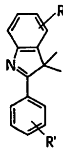
phenylindoles
