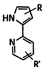
pyridylpyroles
